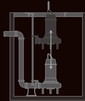
QDC installation
